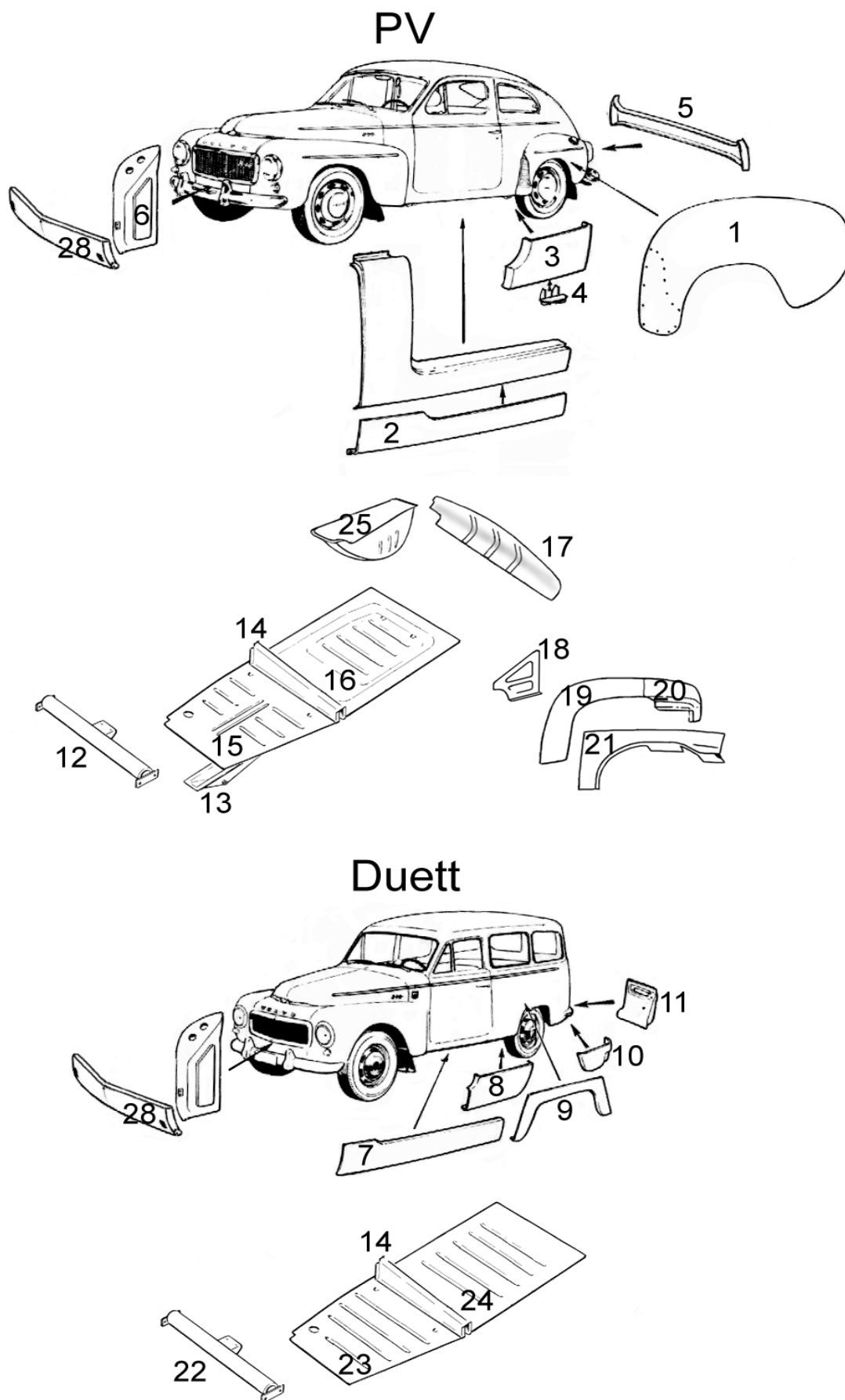
Fig 7: Sheet Metal Parts and Fenders PV/Duett
