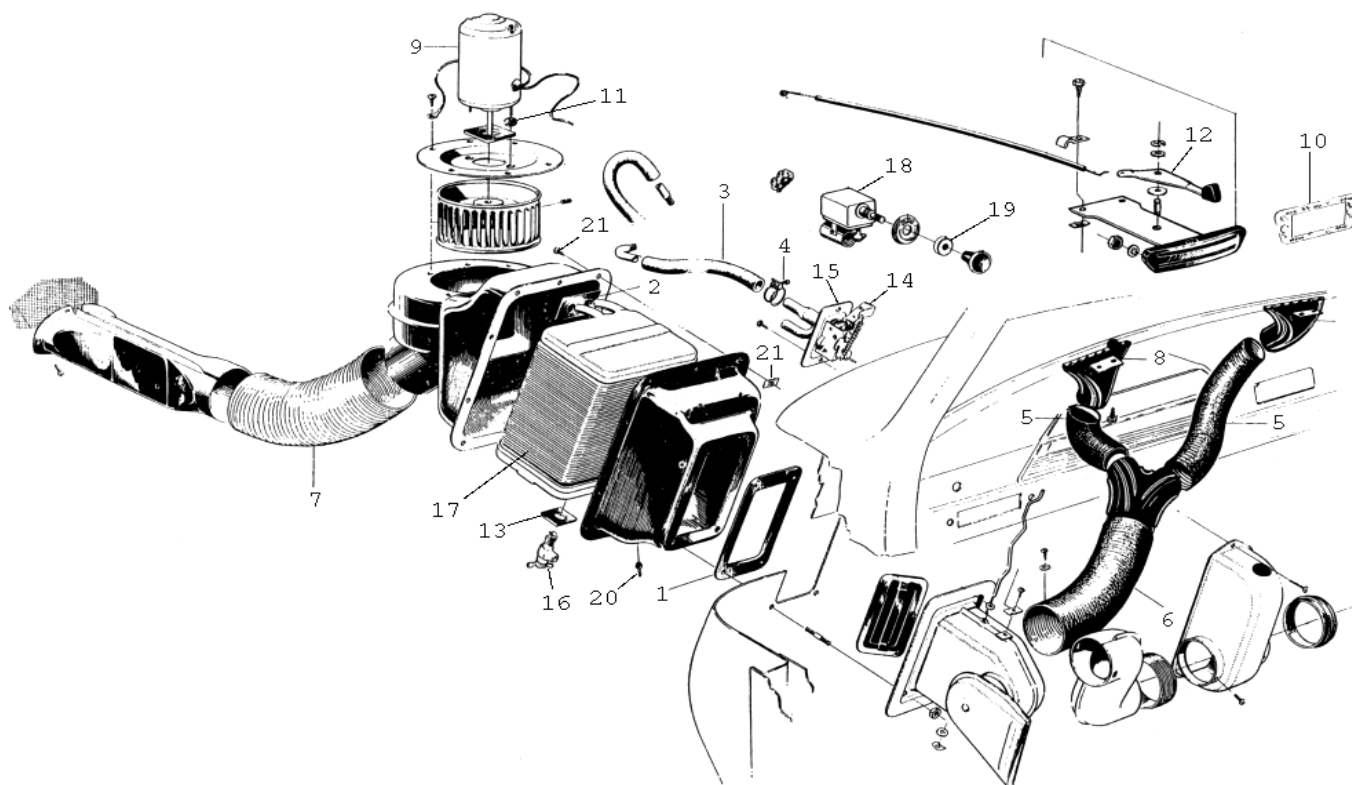
Fig. 2: Heater system
