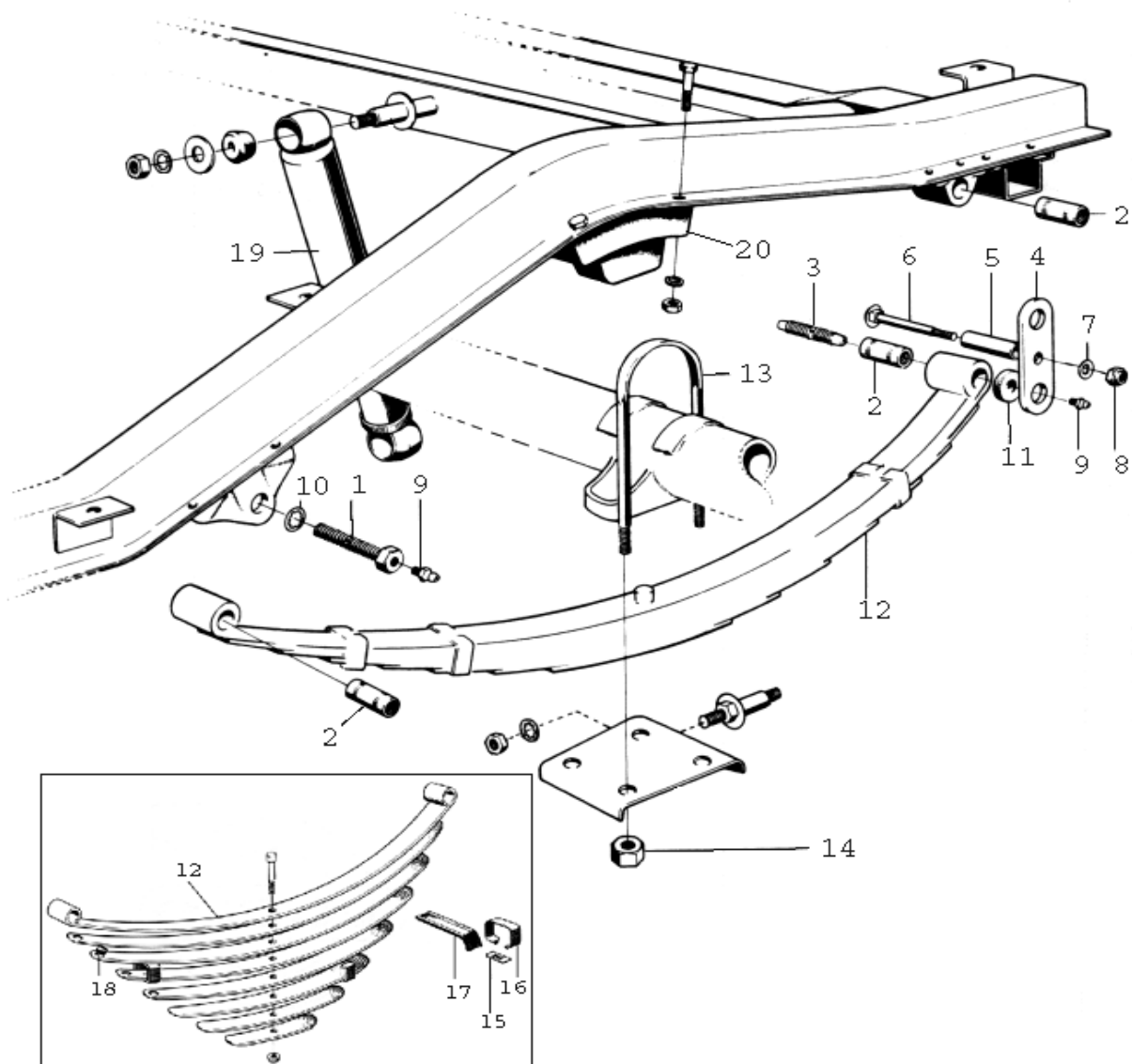
Fig. 5: 210 Rear suspension
